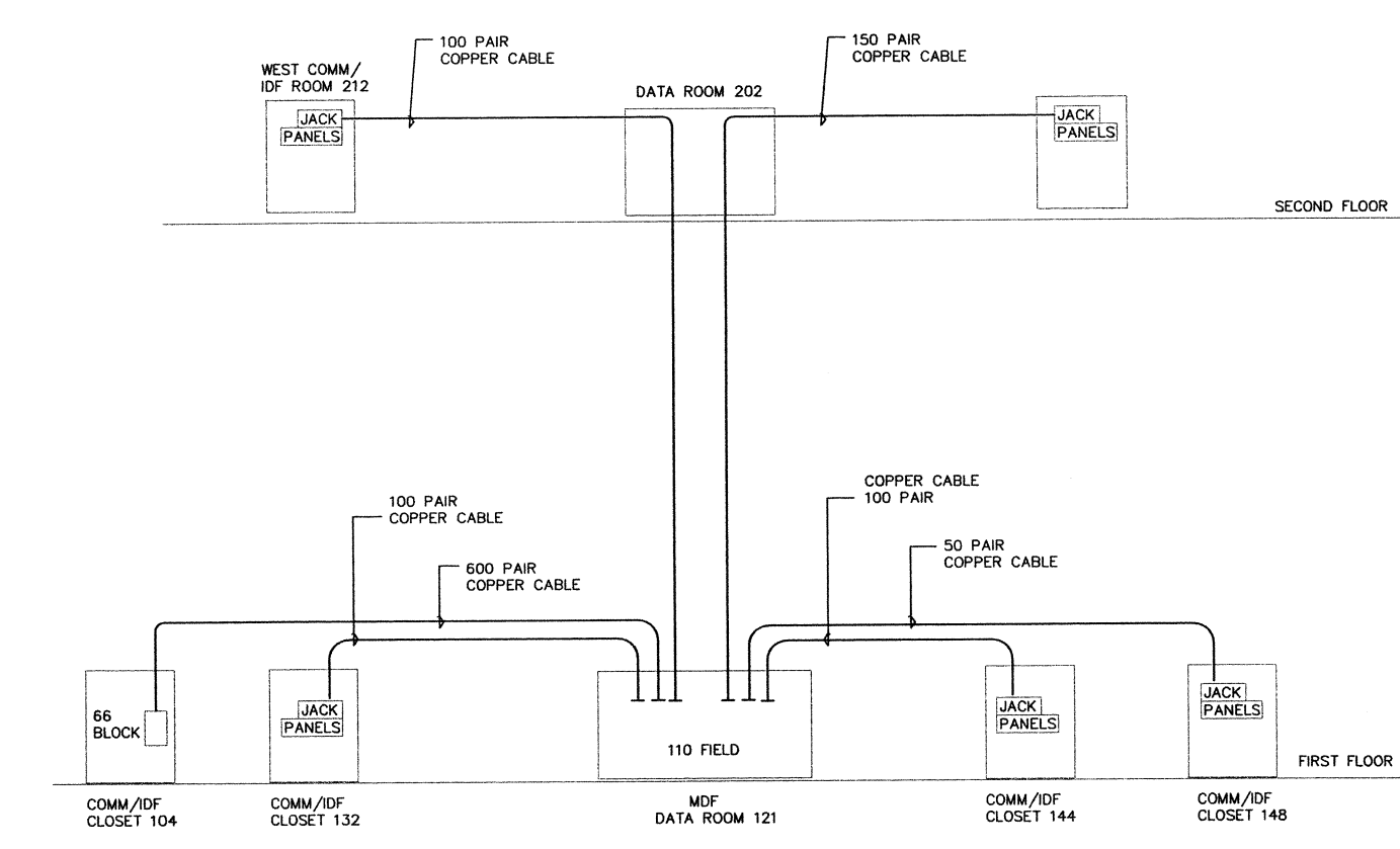
COPPER CABLE DIAGRAM
